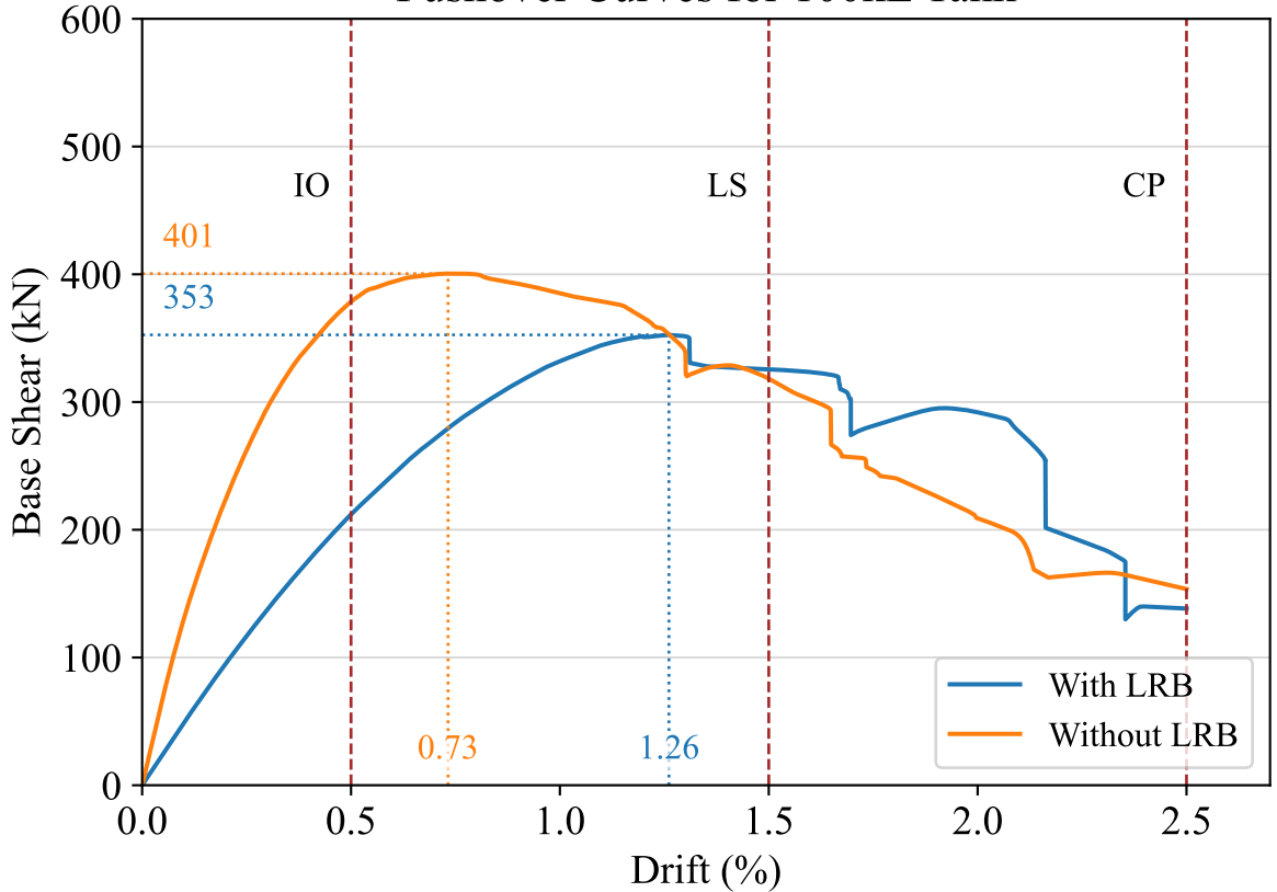
Pushover Curves for 100kL Tank
